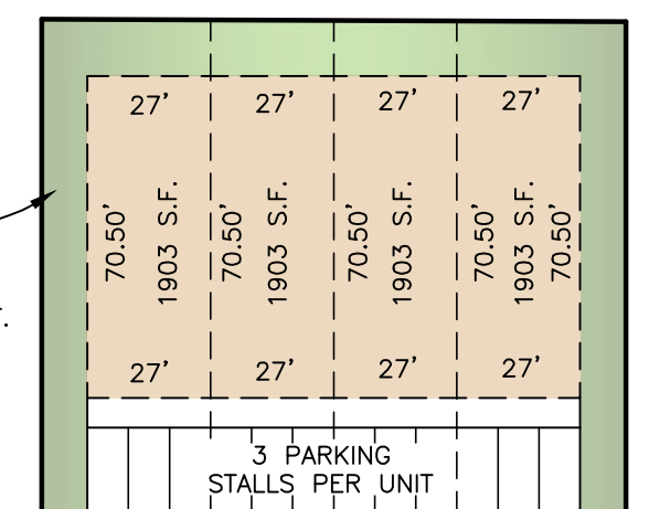
TYPICAL TOWNHOWN DETAIL NO SCALE
